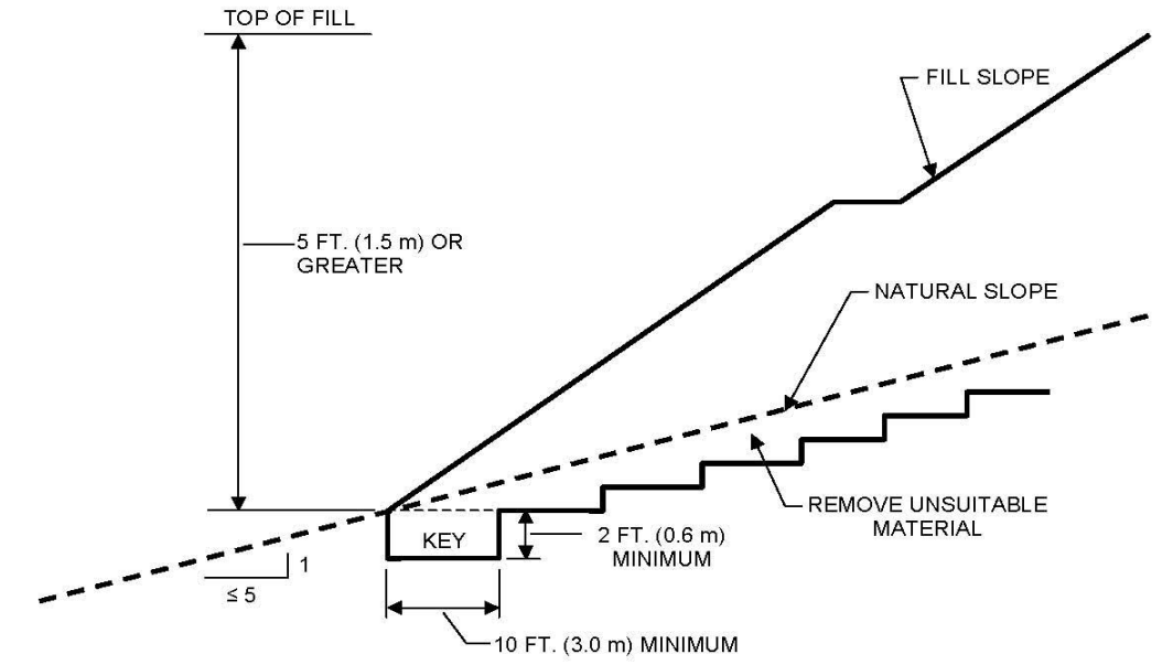
FIGURE J108.3 BENCHING DETAILS
