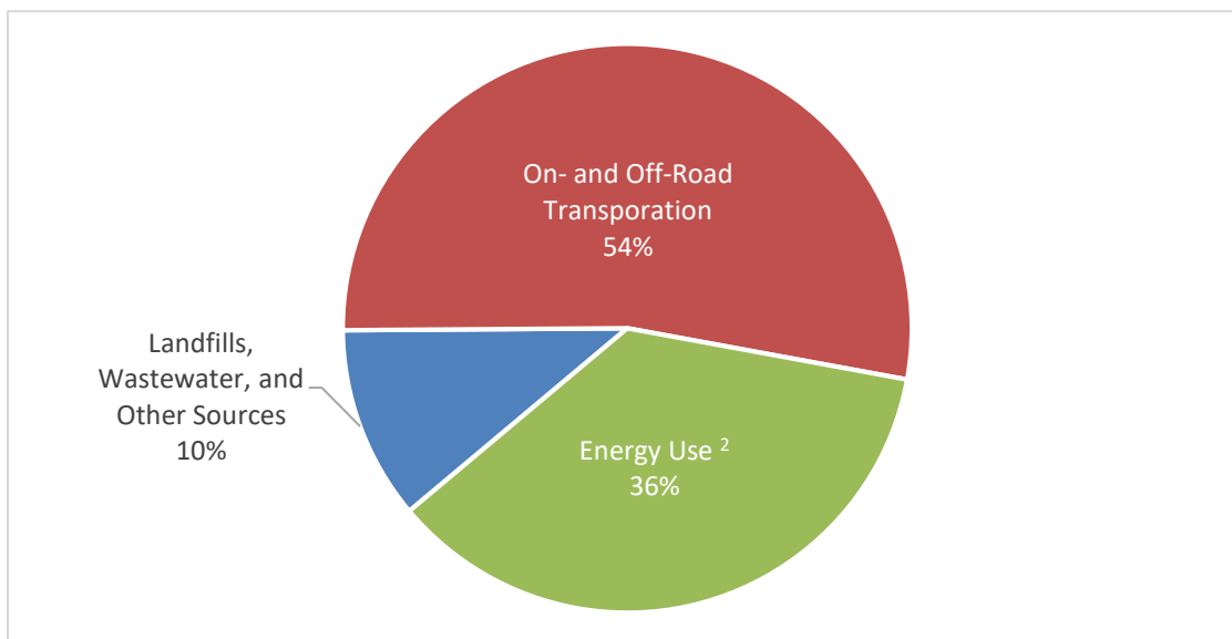
FIGURE 12-1 COUNTYWIDE GREENHOUSE GAS EMISSIONS 1 Ventura County 2012
